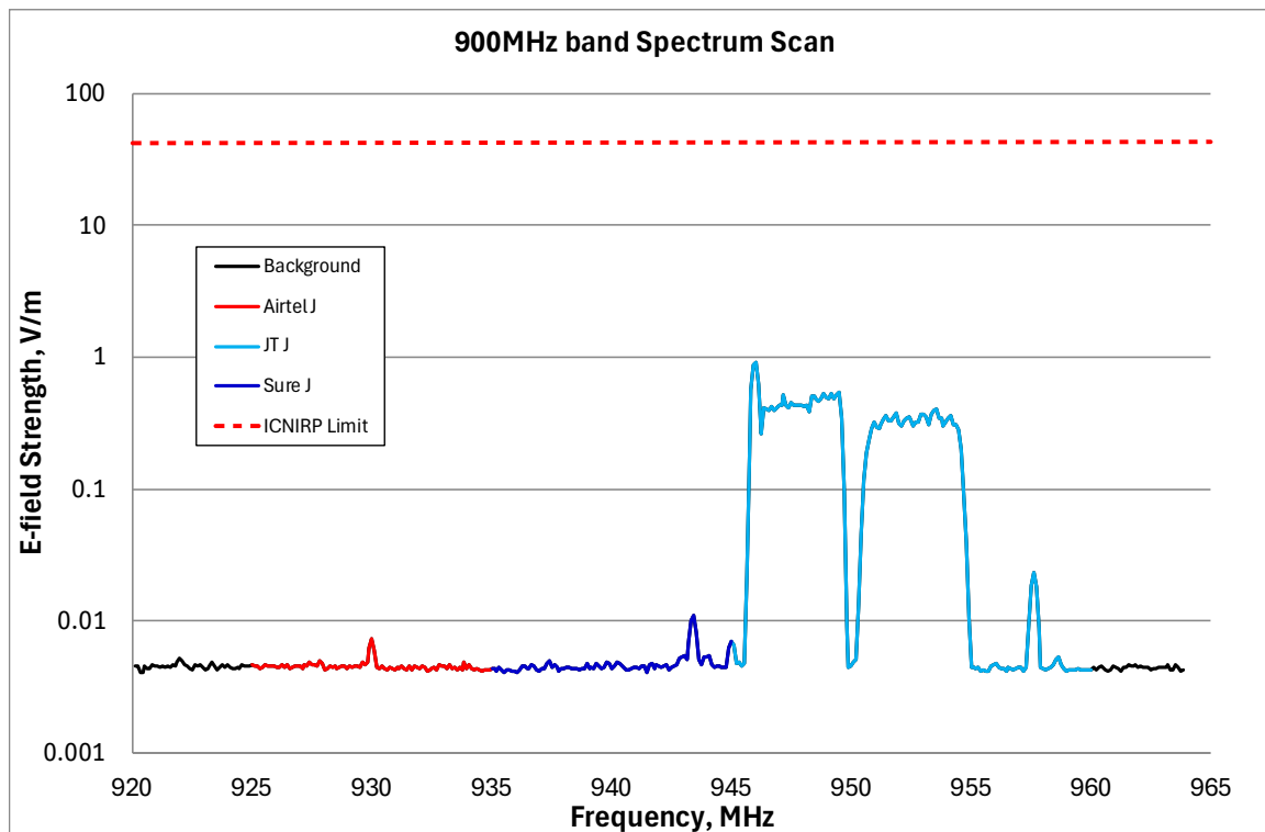
Figure 6 – 900MHz band spectrum scan
