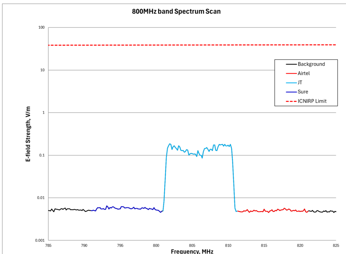
Figure 5 – 800MHz band spectrum scan
