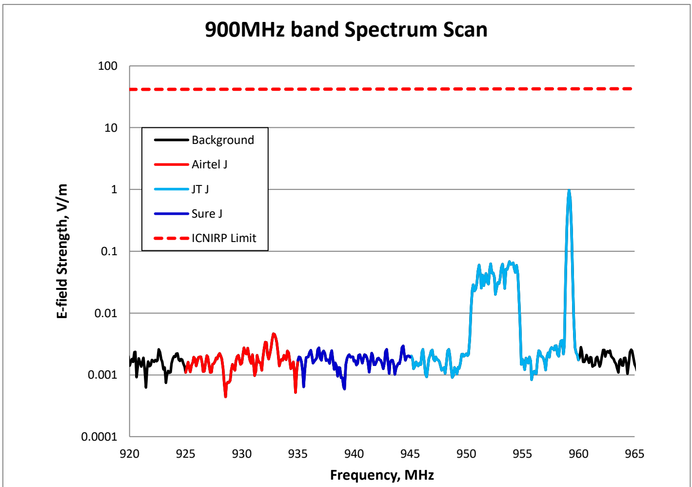
Figure 5 - 900MHz band Spectrum Scan
