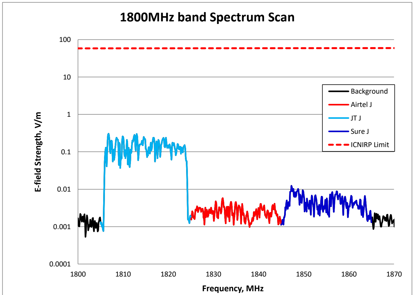
Figure 6 - 1800MHz Spectrum Scan
