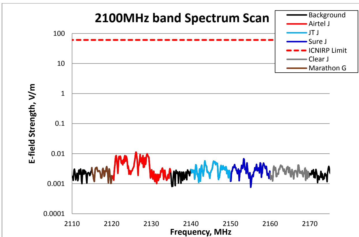
Figure 7 - 2100MHz Spectrum Scan
