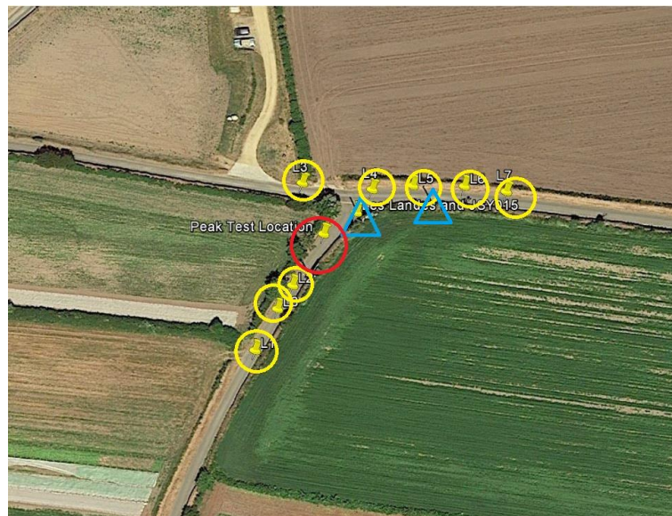
Figure 3- Survey Area with Spot Measurement Markers: The blue triangles are the site locations, the yellow circles are intermediate locations measured at during the peak search and the red circle is the spot where the highest spot search reading was obtained and where the detailed survey was carried out
